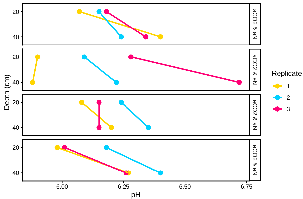
CO 2 xNxPhrag: Porewater pH by Replicate
